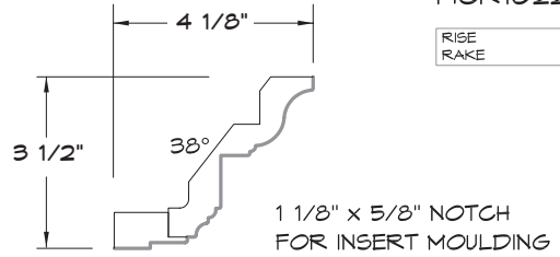
CROWN MOULDING
