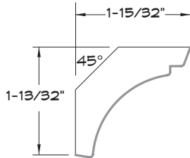
CROWN MOULDING
