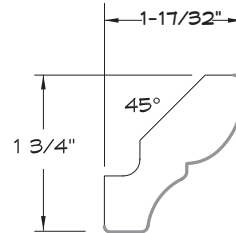
CROWN MOULDING
