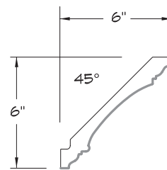
CROWN MOULDING
