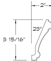
CROWN MOULDING
