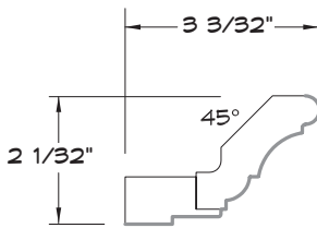
CROWN MOULDING
