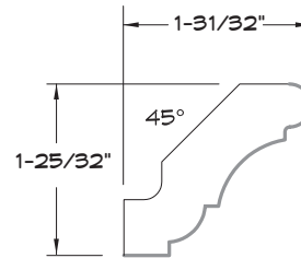
CROWN MOULDING
