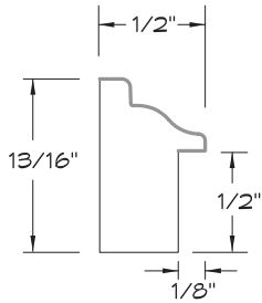
CAP MOULDING
