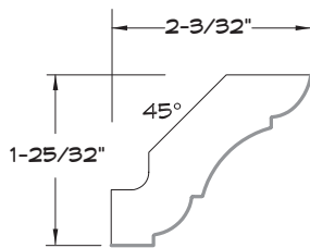
CROWN MOULDING
