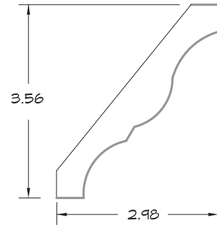
ROYAL CROWN 1309
