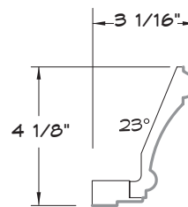
CROWN MOULDING
