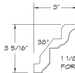
CROWN MOULDING
