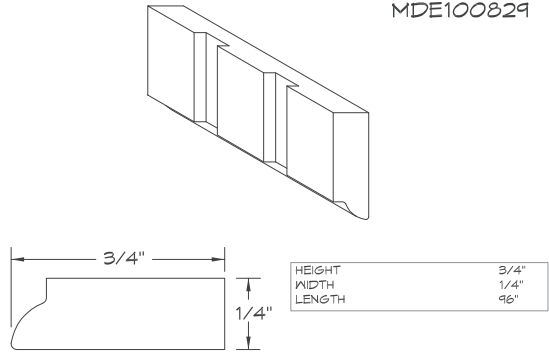
DENTIL MOULDING
