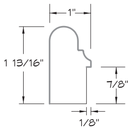
CAP MOULDING
