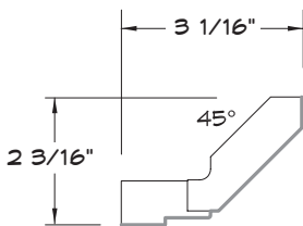
CROWN MOULDING
