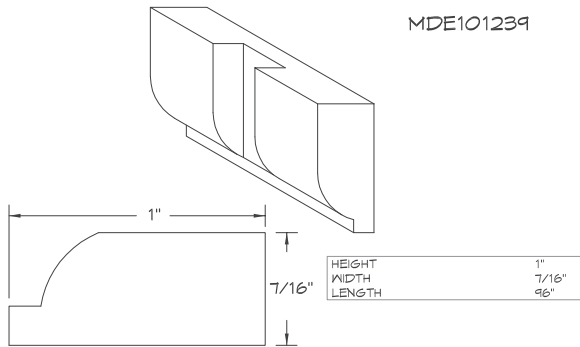
DENTIL MOULDING
