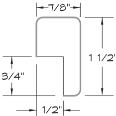
RETAINER MOULDING
