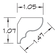
SOFFIT CROWN 1310
