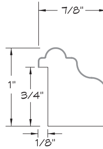
CAP MOULDING
