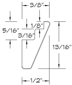
ASTRAGAL MOULDING
