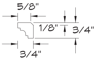
INSIDE CORNER MOULDING # MIC100108
