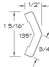
OUTSIDE CORNER MOULDING
