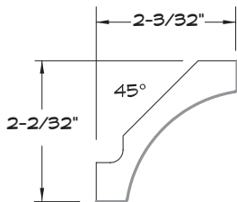
CROWN MOULDING
