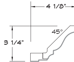
CROWN MOULDING
