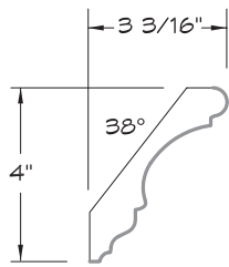
CROWN MOULDING
