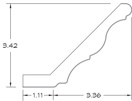
DESIGNER CROWN 1305
