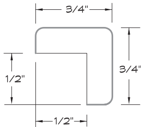
OUTSIDE CORNER MOULDING
