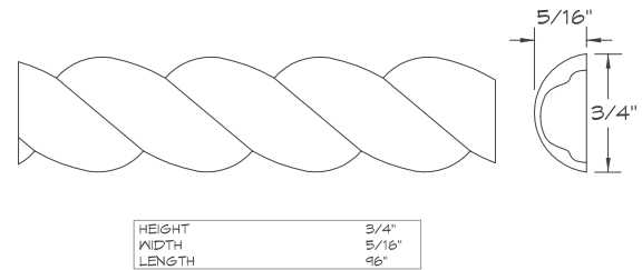
ROPE MOULDING
