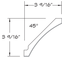
CROWN MOULDING
