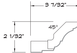
CROWN MOULDING
