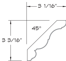
CROWN MOULDING
