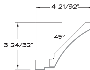
CROWN MOULDING
