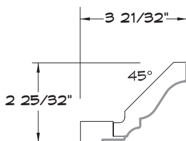
CROWN MOULDING
