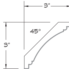
CROWN MOULDING
