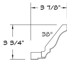
CROWN MOULDING
