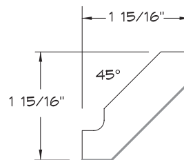
CROWN MOULDING
