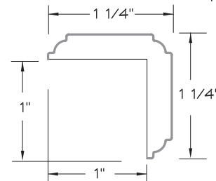
OUTSIDE CORNER MOULDING
