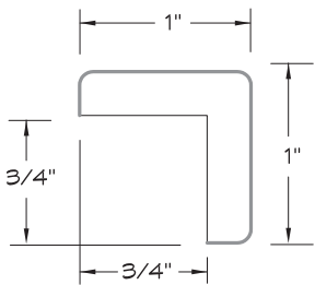
OUTSIDE CORNER MOULDING
