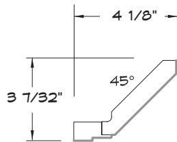
CROWN MOULDING
