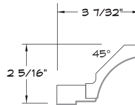
CROWN MOULDING
