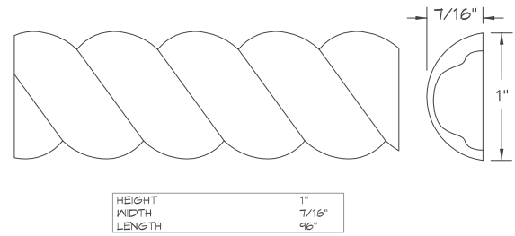
ROPE MOULDING
