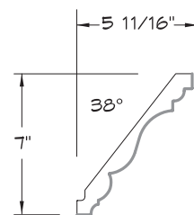
CROWN MOULDING
