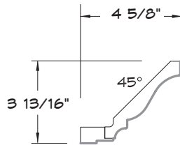
CROWN MOULDING
