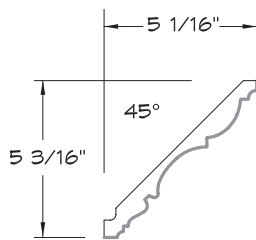
CROWN MOULDING
