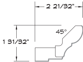
CROWN MOULDING
