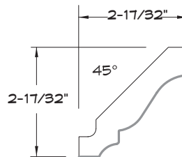
CROWN MOULDING
