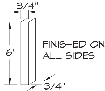
CORNER BLOCK TRANSITION MOULDING # MTB000CBT
