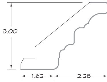
REGAL CROWN 1306
