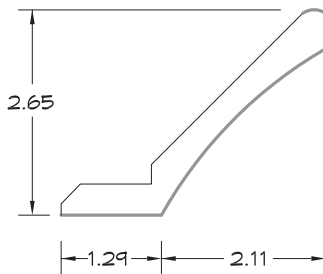
COVE CROWN 85023
