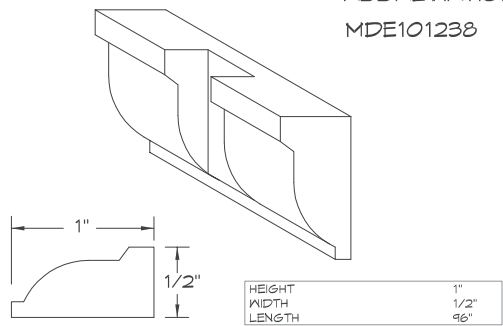
DENTIL MOULDING
