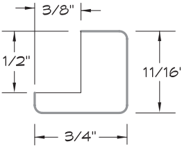
RETAINER MOULDING
