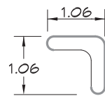
OUTSIDE CORNER 1407
