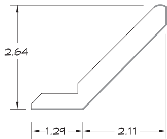
STRAIGHT CROWN 85024
